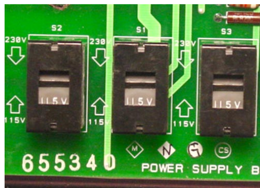
Figure 2-1. Power Supply Board Voltage Select Switches
